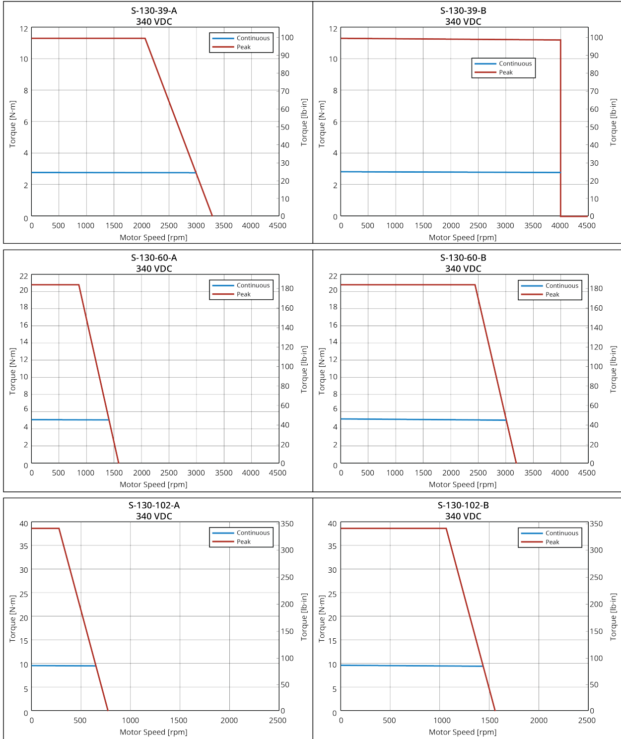
Figure 1-3: Torque Speed Curves (S-130-XX)
