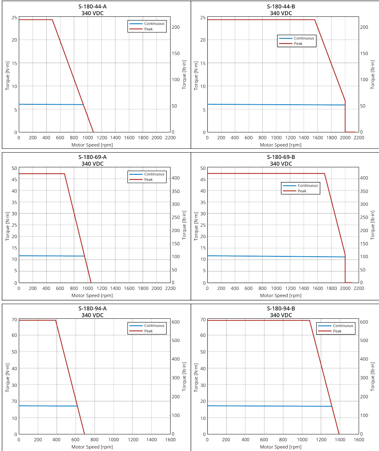
Figure 1-4: Torque Speed Curves (S-180-XX)
