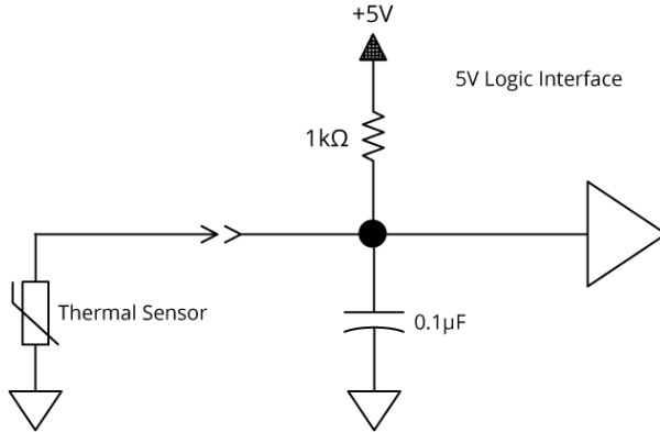
Figure 2-6: Typical Thermistor Interface Circuit
