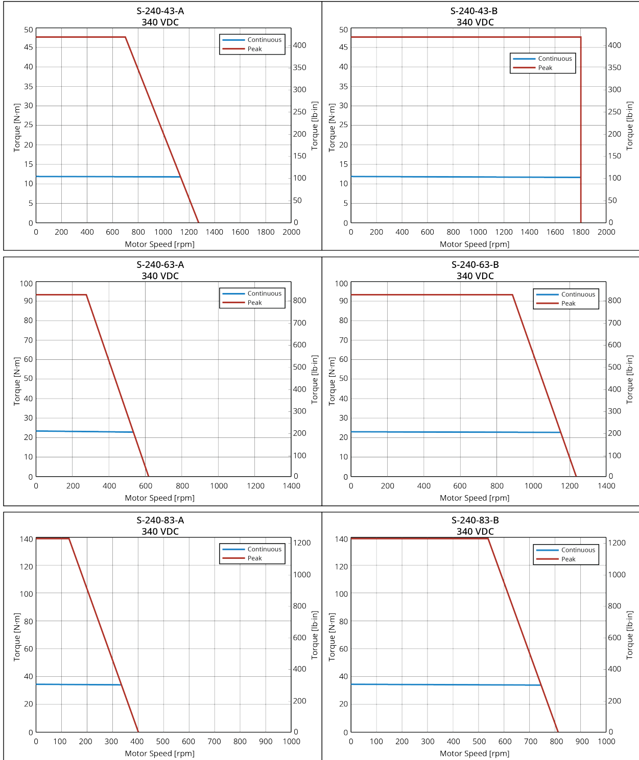
Figure 1-5: Torque Speed Curves (S-240-XX)
