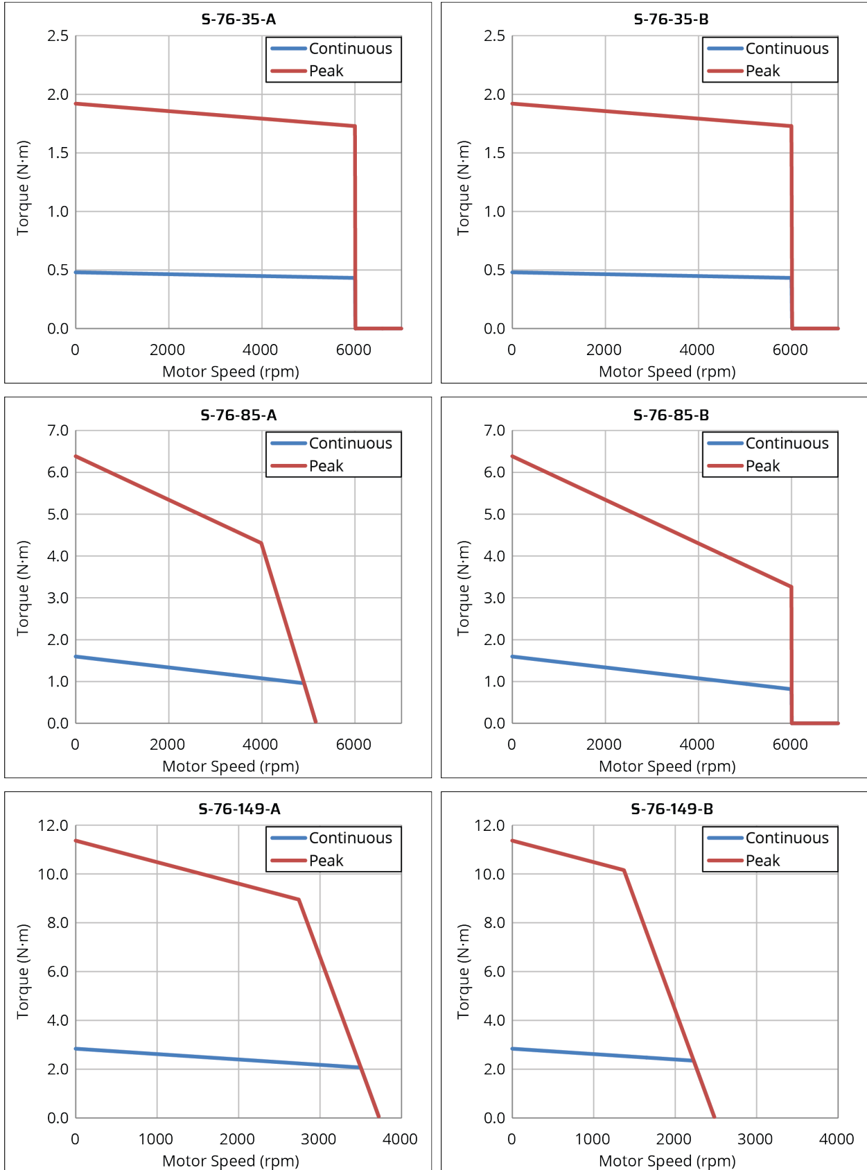
Figure 1-2: Torque Speed Curves (S-76-XX)
