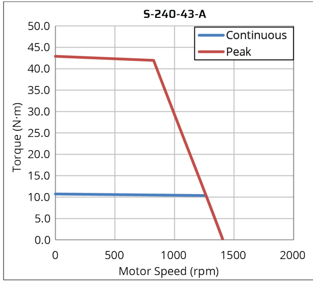
Figure 1-5: Torque Speed Curves (S-240-XX)
